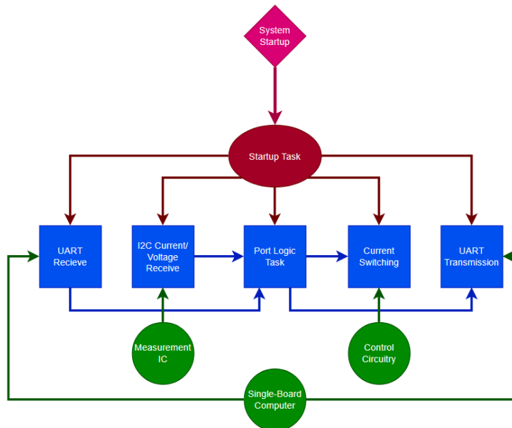
Figure 7.2a: MCU Task Block Diagram
