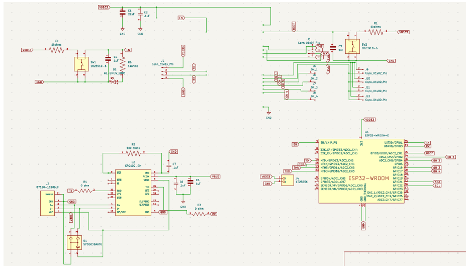
Figure 6.3: Full Schematic of MCU
