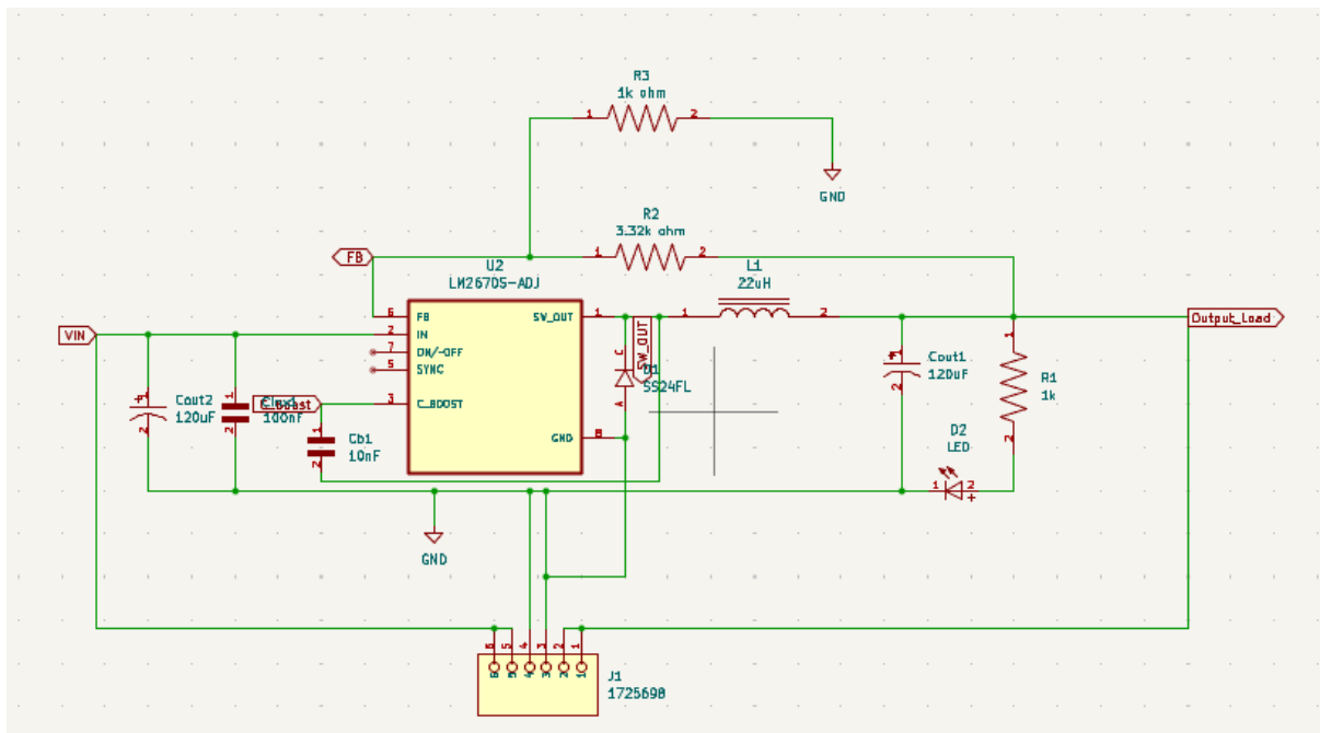
Figure 6.1B: Schematic of 5 Volt Regulator
