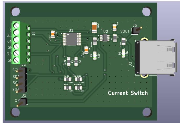
Figure 8.1b: Current Switch Layout
