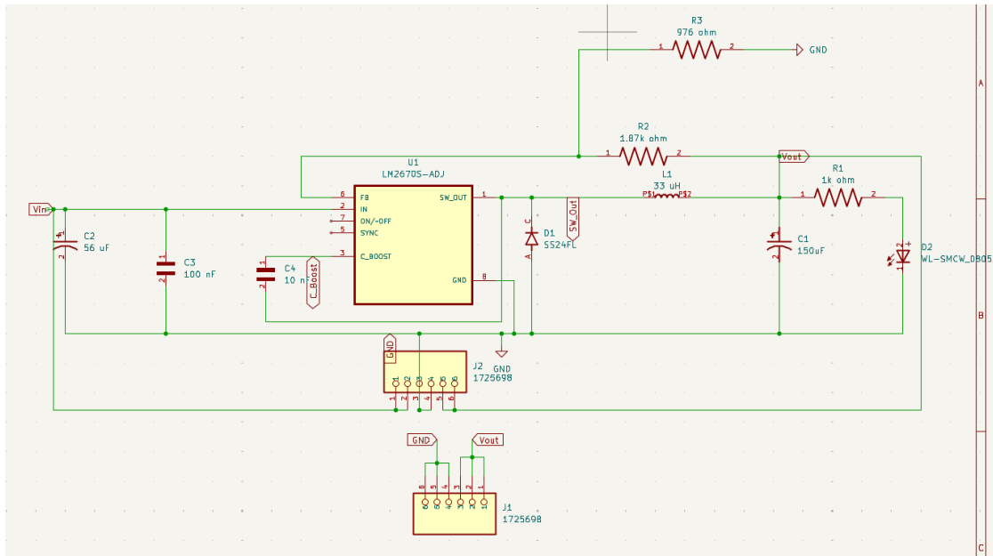
Figure 6.1A: Schematic of 3.3 Volt Regulator
