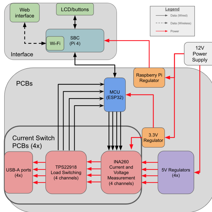
Figure 2.6: Hardware Block Diagram
