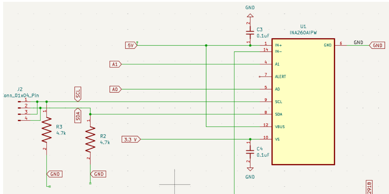
Figure 6.2b: Schematic of INA260 - Current and Voltage Measurement IC
