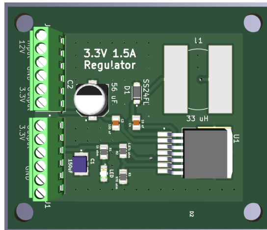
Figure 8.2a: 3.3V Regulator Board
