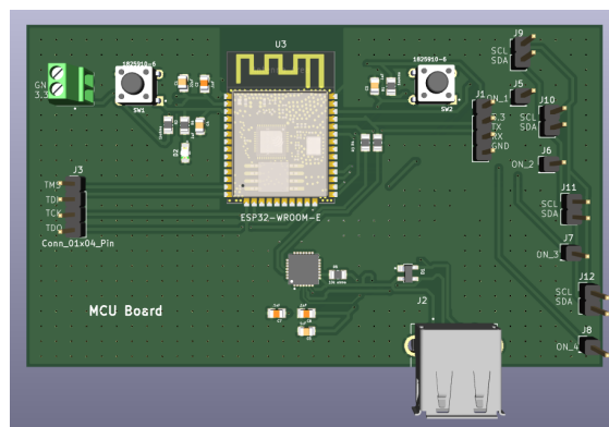
Figure 8.1a: MCU Board
