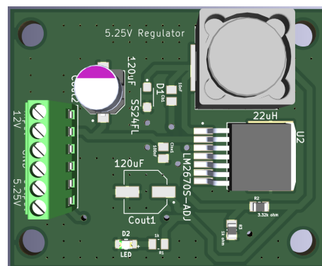
Figure 8.2b: 5V Regulator Board
